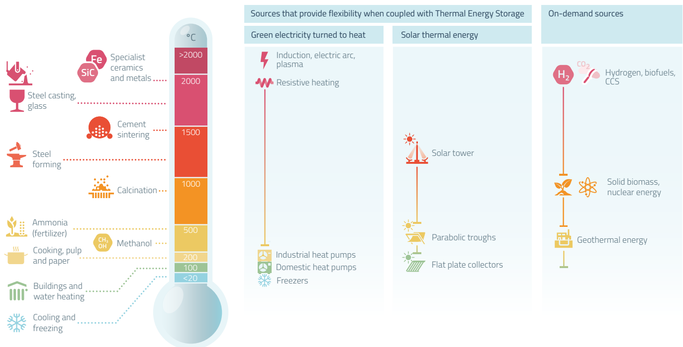
Figure 3: Potential pathways for low-carbon, high-temperature heat. Source: Future Cleantech Architects factsheet on thermal energy storage [13]
