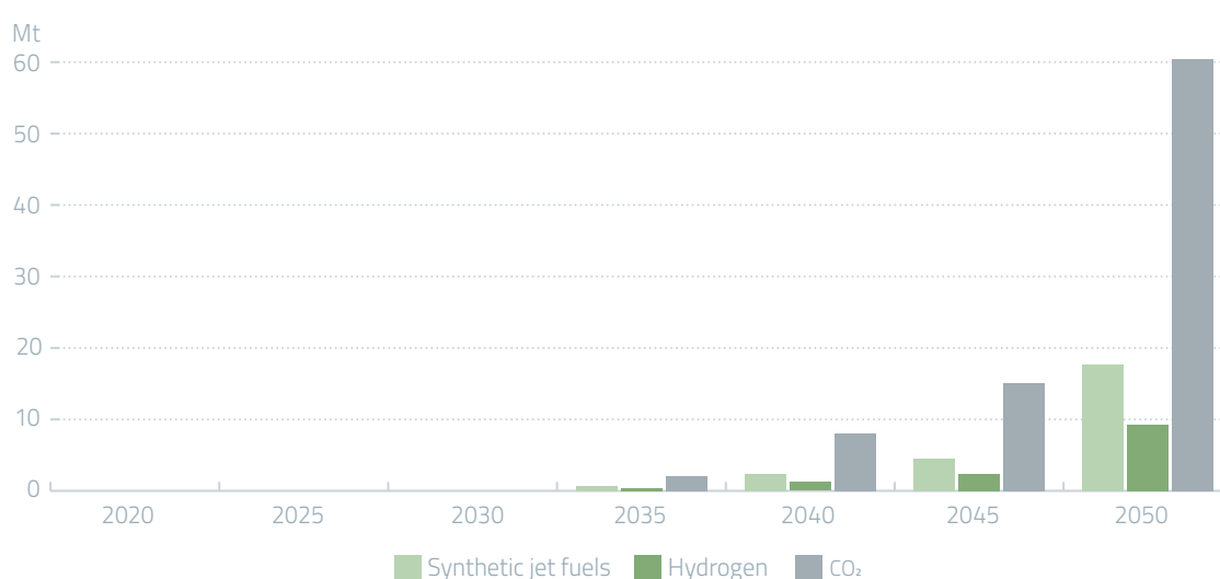
Figure 7: The amount of CO 2 and hydrogen needed to produce the requisite minimum amount of synthetic jet fuels until 2050 per the subtargets of ReFuelEU Aviation.
