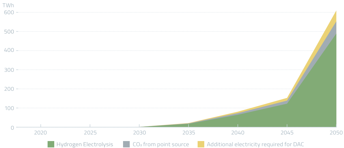
Figure 8: The renewable electricity required to produce hydrogen via electrolysis, CO 2 from point source CCU, and the additional electricity needed if CO 2 from DAC were opted for over point source CCU.
